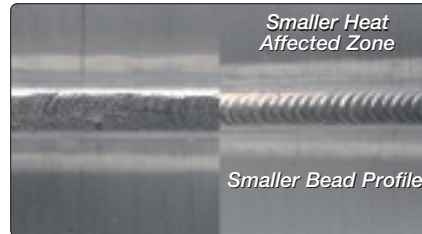
Standard TIG Weld (at 60 amps) Pulsed TIG Weld (at 60 amps)
