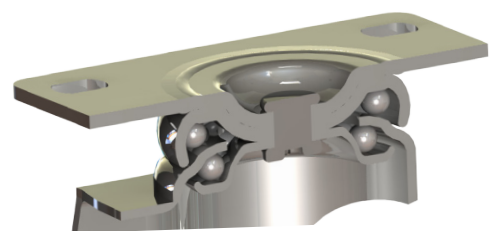
CROSS SECTION LIGHT INDUSTRIAL SERIES PLATE TYPE CASTOR
