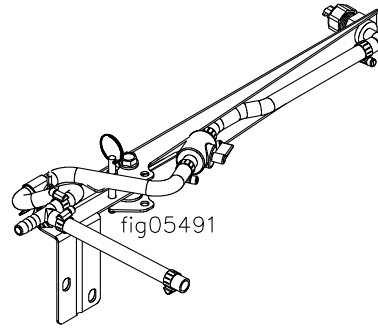
Left Broadcast Boom Assembly (Qty 1)
