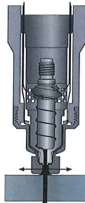
LC105 torch design with drag cup
