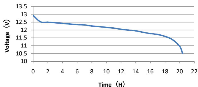
20hr Capacity (25°C) test
