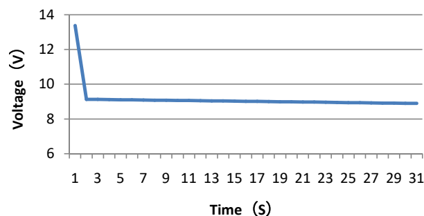
-18°C Cold cranking test (600CCA)
