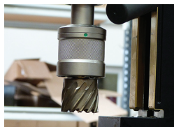
Cutter held in chuck
