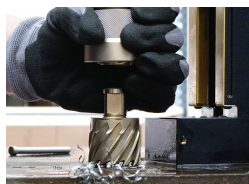
Cutter released
