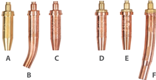
OXY/ACETYLENE
