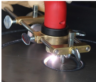
Circle Guide - Plasma
