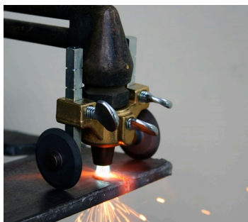
Roller Guide - Gas
